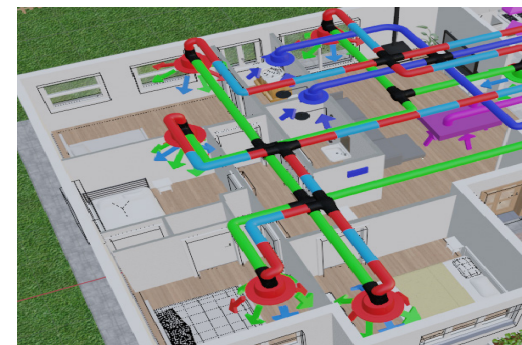
In Ceiling system layout
